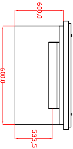
Rain Cover 600 L Artikalnř: 7172064
