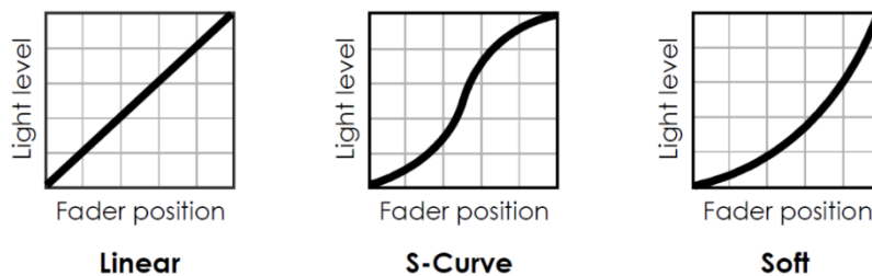
Figure 4. Dimming curves
