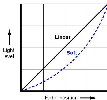
Figure 2. Dimming curves
